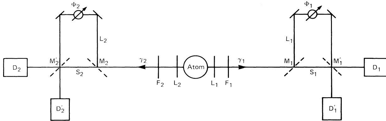
FIG. 2. Photon coincidence measurements including interference between the amplitudes along the shorter paths, S_1 and S_2 , and the longer paths, L_1 and L_2 .
