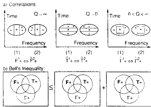
Fig. 2. (a) Expected correlations in measurements of the "windowed" time-dependent spectrum, as in eqs. (4). (b) Bell inequality (6), with assumptions of eqs. (4) and (5).
