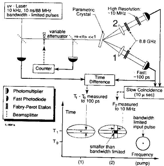
Fig. 1. Possible E-P-R experiment using time and frequency measurements on parametrically generated photons.
