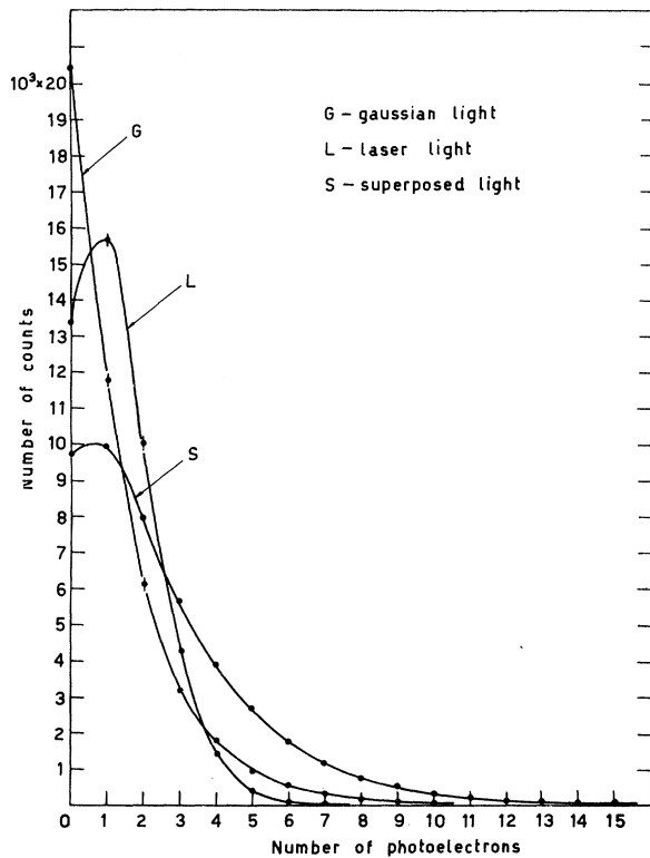
FIG. 1. Photocount distributions for Gaussian, laser, and superposed field. Measuring time of a single sample: 10 \mu sec. Coherence time of the Gaussian field: 40 \mu sec.
